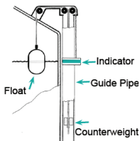
LIQUIDATOR 2 LEVEL GAUGE
